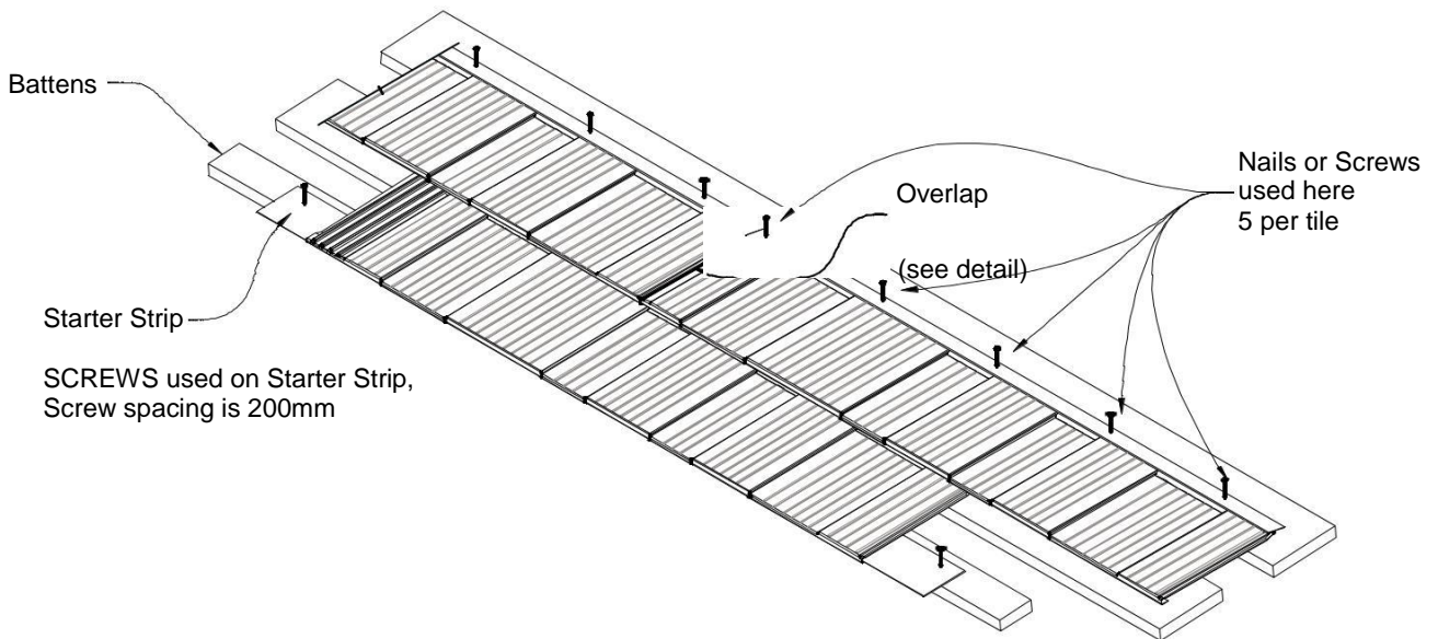
Fastening Detail
