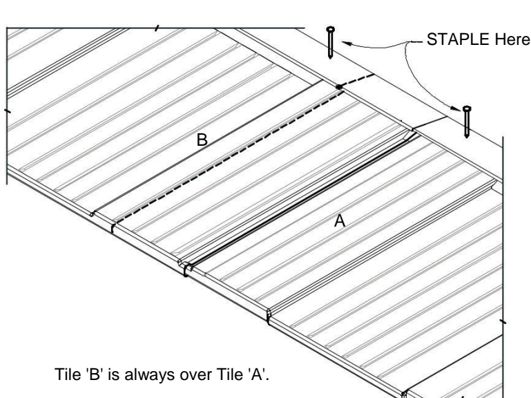
Overlap Detail
