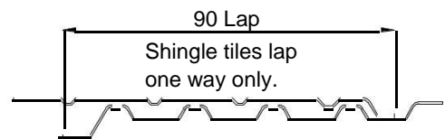
Lap Section
