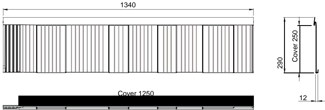
Tile Dimensions
