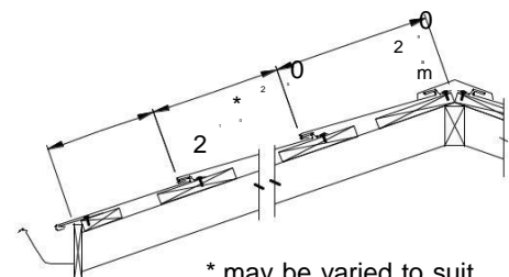
Batten Layout
